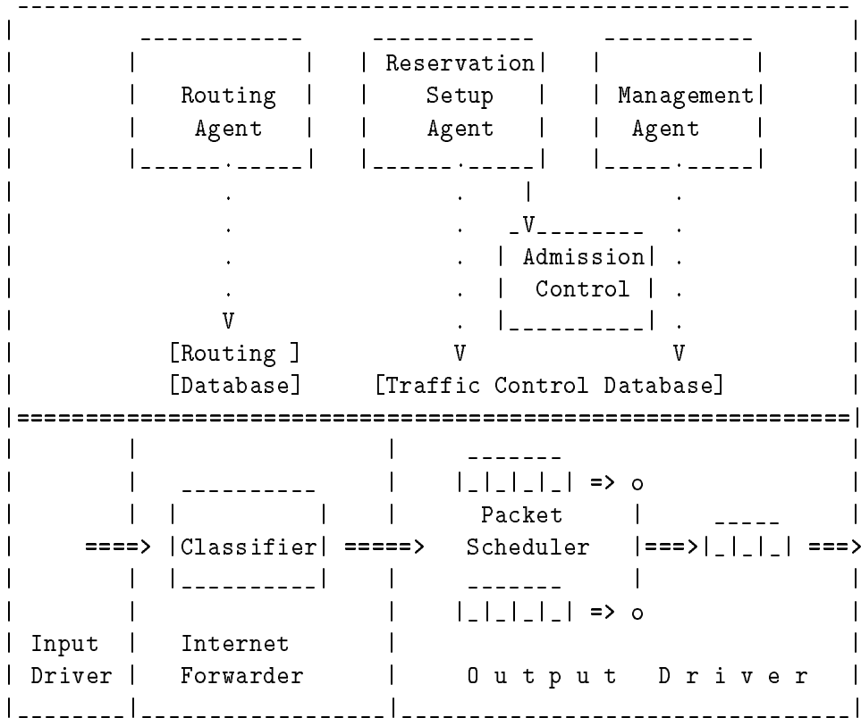
Figure 1: Implementation Reference Model for Routers
